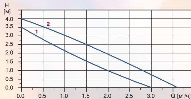
SOLAR 25-40
