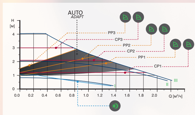
ALPHA2 25-40, ALPHA2 32-40
