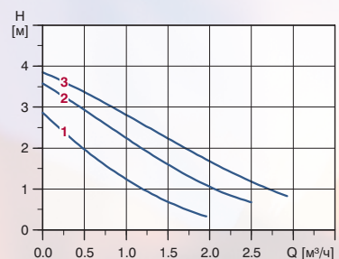
UPS 25-40 UPS 32-40 180
