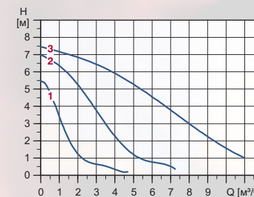
UPS 32-80 180
