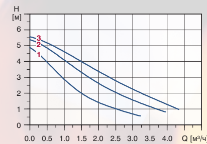
UPS 25-60 UPS 32-60 180
